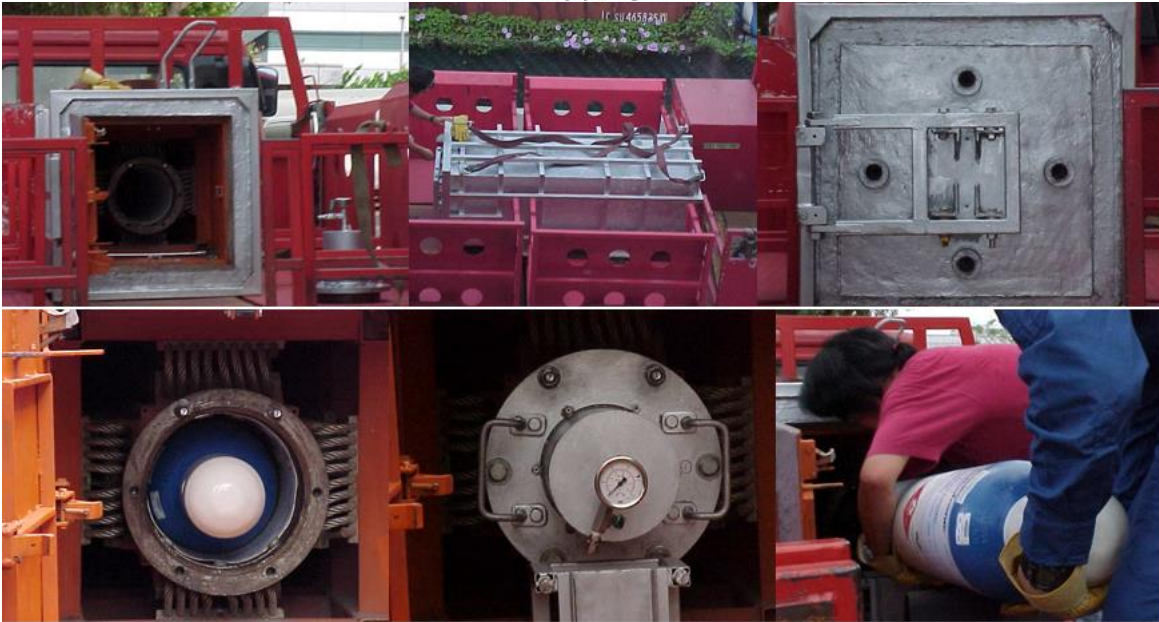
Fig. 1: ERCV in a Fire Proof Enclosure
